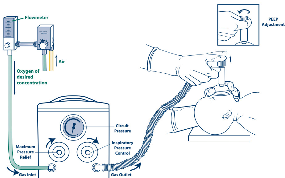
Figure 3.4. Flow-controlled, pressure-limited device (T-piece resuscitator). Pressures are pre-set by adjusting controls on the device and are delivered by occluding and opening the aperture in the PEEP cap.
